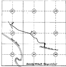
County Road CHANGE IN LINKVILLE AND TULE LAKE ROAD Scale 1/4" = 100 Feet 1/4" = 3300 Feet Surveyed June 1883 by J.B. Griffith, County Surveyor See Road Record Vol 1 pg 63 Compiled September 1912 "X" indicates section lines
